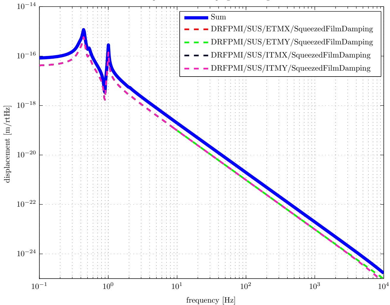
Squeezed Film Damping NoiseBudget
