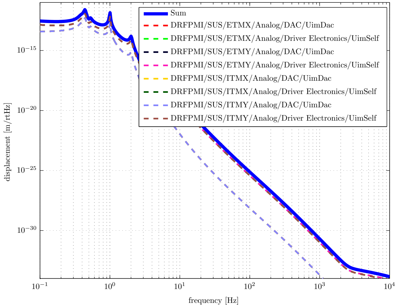
QUAD L1 NoiseBudget
