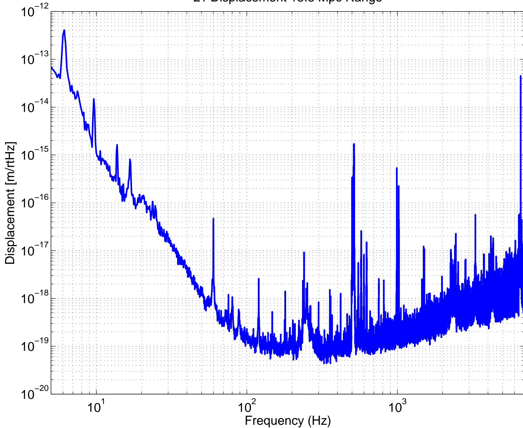
L1 Displacement 15.8 Mpc Range
