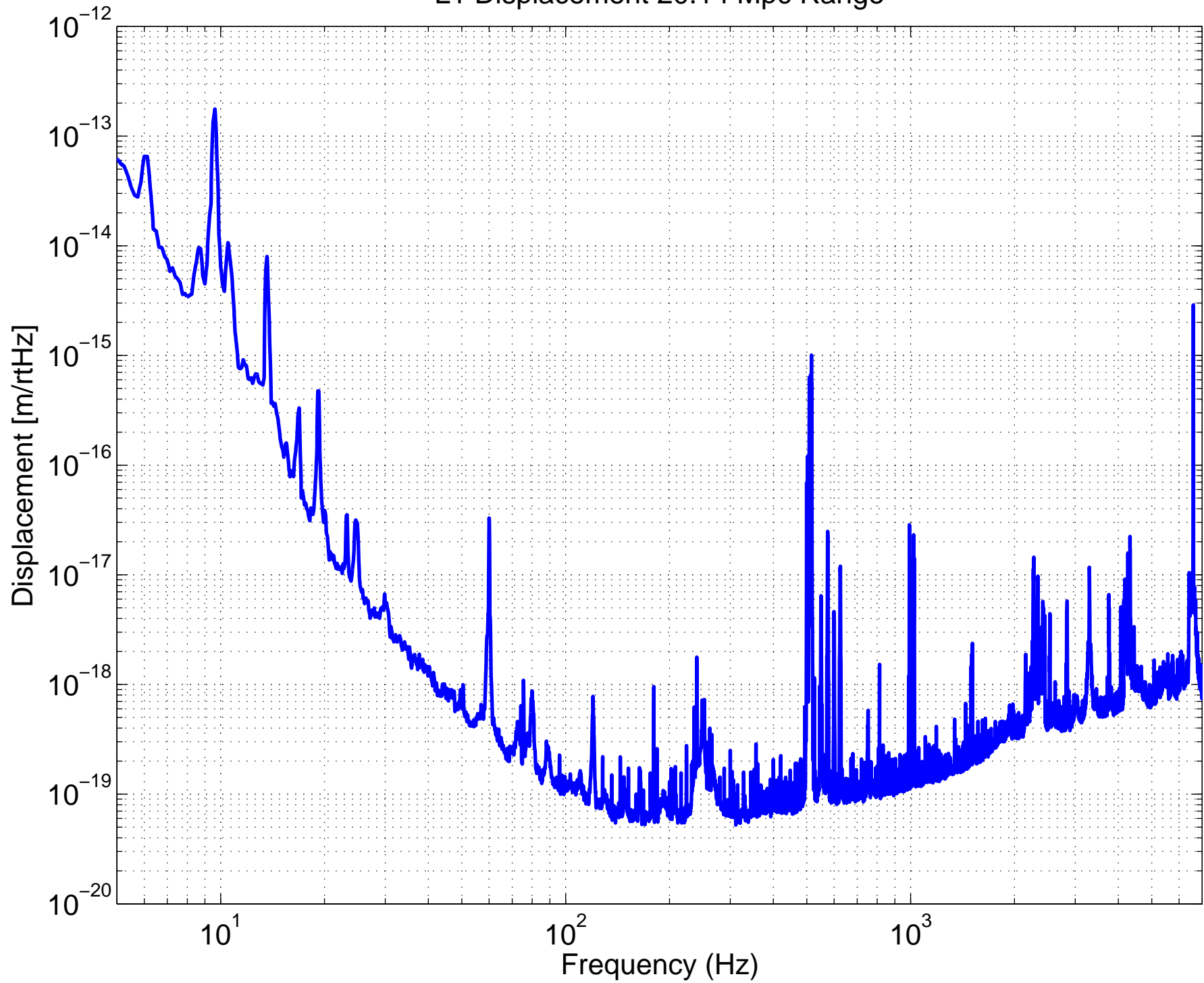
L1 Displacement 20.14 Mpc Range
