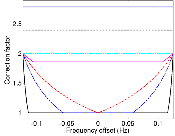
FIG. 8: Simulated correction of \hat{Y}_{\text{tot}} for the Radiometer search across the standard 0.25 Hz-wide bin for a variety of frequencies. Bin center falls at the frequency offset of 0 Hz. The traces, from bottom to top, display the simulation for 40 (black, solid), 290 (blue, dashed), 538 (red, dot-dashed), 1000 (magenta, solid), 1076 (cyan, dashed), 1290 (black, dot-dashed), and 1500 Hz (blue, solid). Below 538 Hz note that at the bin boundary, where only half of the SNR is in this bin, the correction factor is two. The correction factor is one when the signal is completely within the bin. \Delta f is larger for 290 Hz than for 40 Hz, thus the frequencies at which the injection is completely within the chosen bin (and thus has a correction factor of one) are fewer. Above 538 Hz, it is not possible to have the entire injection within a single frequency bin df . At most, df/\Delta f of the injection can be within a single bin, resulting in a correction factor that is always greater than one. Above 1076 Hz, \hat{Y}_{\text{tot}} is always df/\Delta f of the injection.
