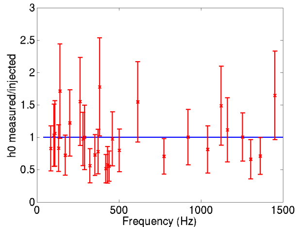
FIG. 10: Ratio of measured and corrected to injected h_0 for the Radiometer search for the open signals. An extra empirical factor of \sqrt{3} has been included in the uncertainties. When the measured and the injected h_0 agree to within one standard deviation, the error bars for the data (red) should intersect the blue line which has a value of one.
