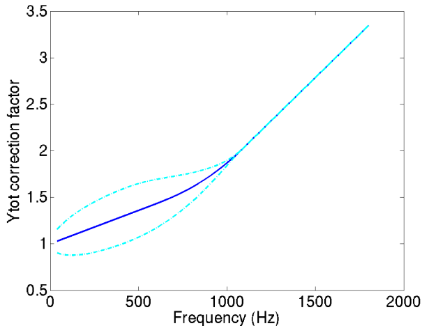
FIG. 9: Frequency bin correction factor necessary to account for signals spanning multiple bins in the Radiometer search.
