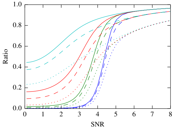
FIG. 3. Ratio between Fisher matrix elements (solid: \hat{\mathbf{\Omega}}_{\gamma\gamma} , dashed: \hat{\mathbf{\Omega}}_{\gamma\tau} , dotted: \hat{\mathbf{\Omega}}_{\tau\tau} ) for the autocorrelation likelihood and the full GW data. Colors correspond to different arrival time priors as in Fig. 2.
