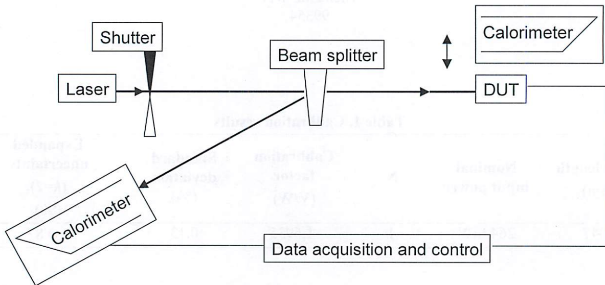
Figure 1. Measurement setup
