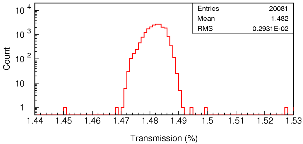
Fig. 1 ITM06 transmission over a 160 mm diameter aperture.
