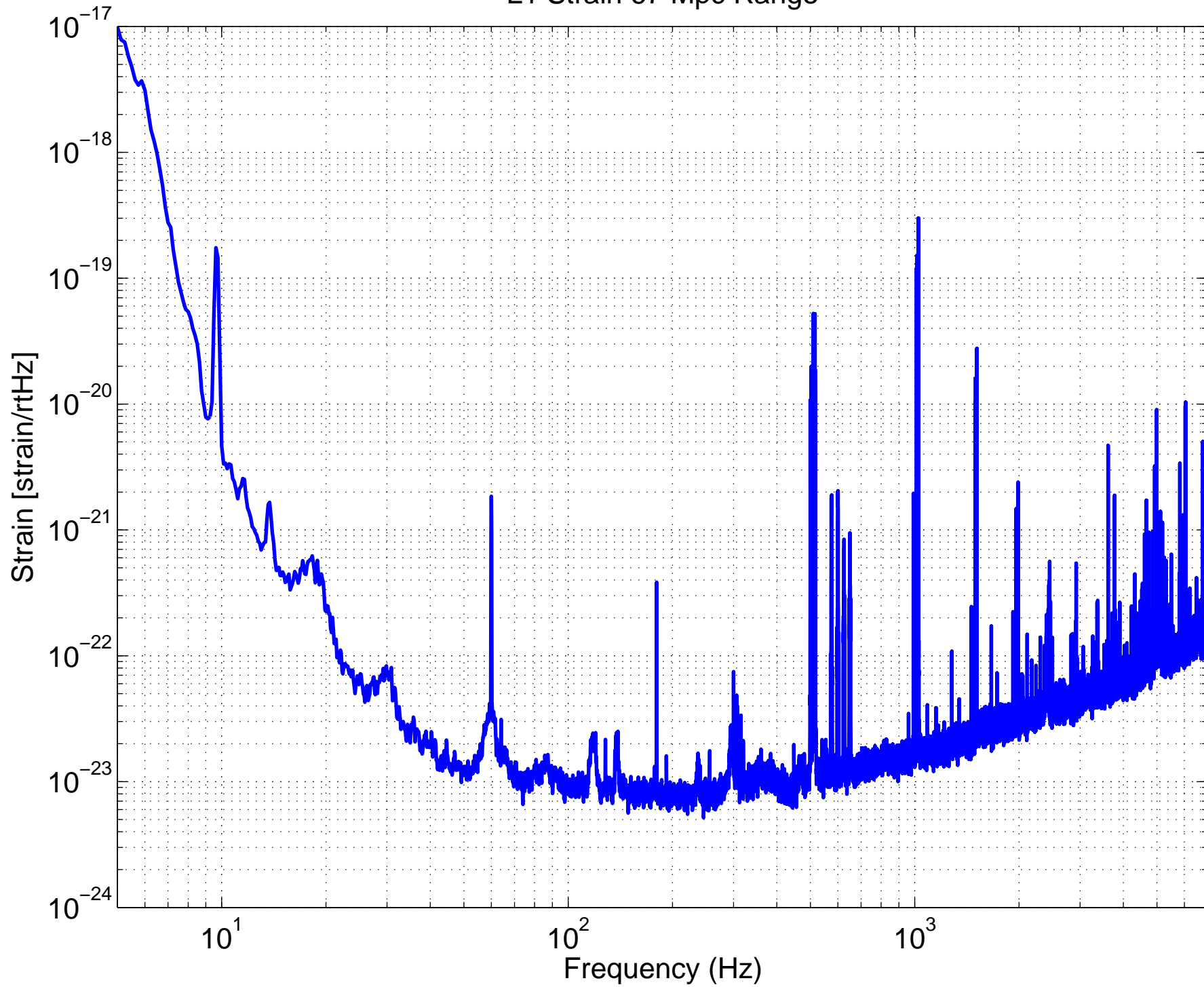
L1 Strain 67 Mpc Range
