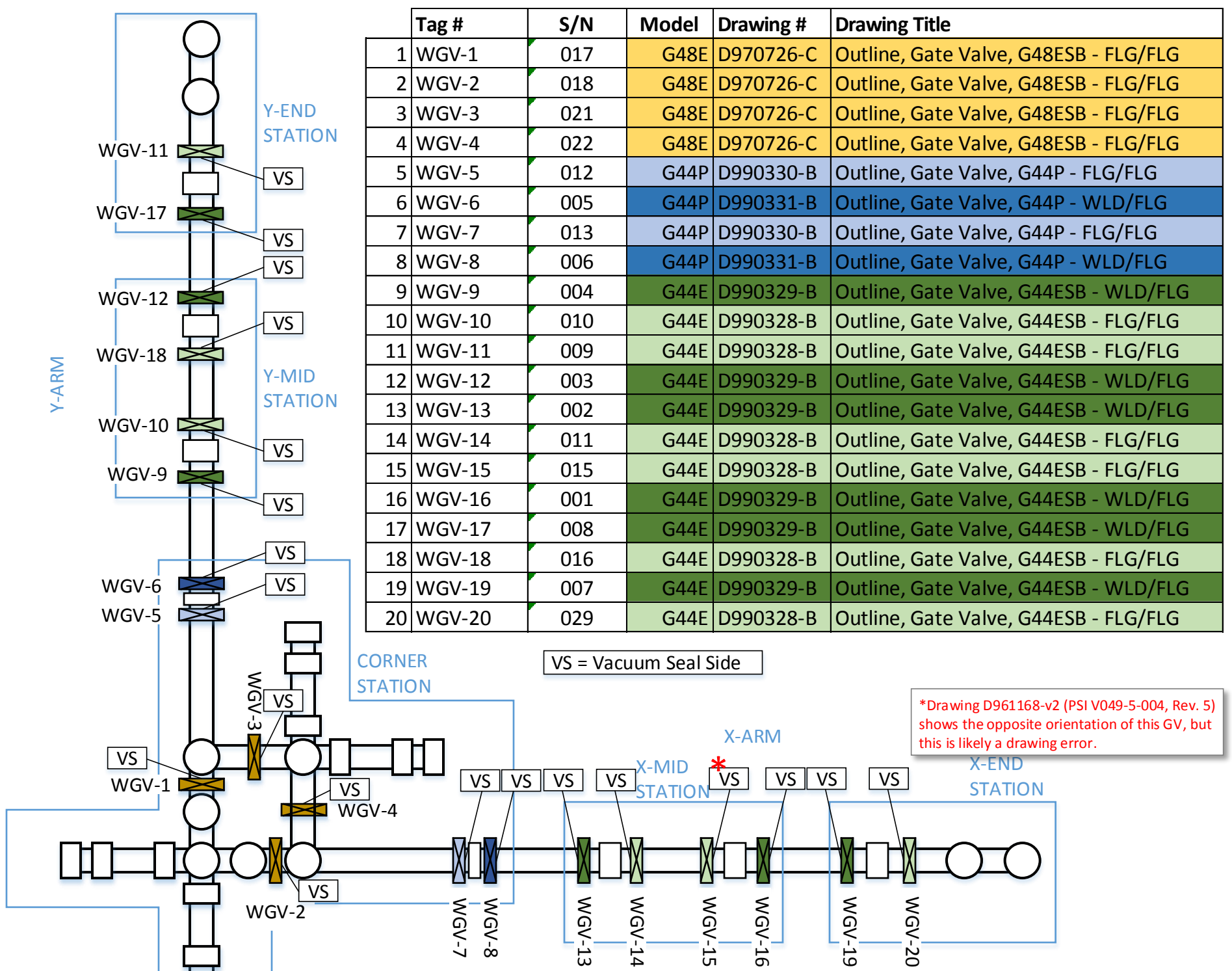
D1600164-v1, Gate Valve Designations, Locations, Orientations and Quantities Sheet1: LHO
