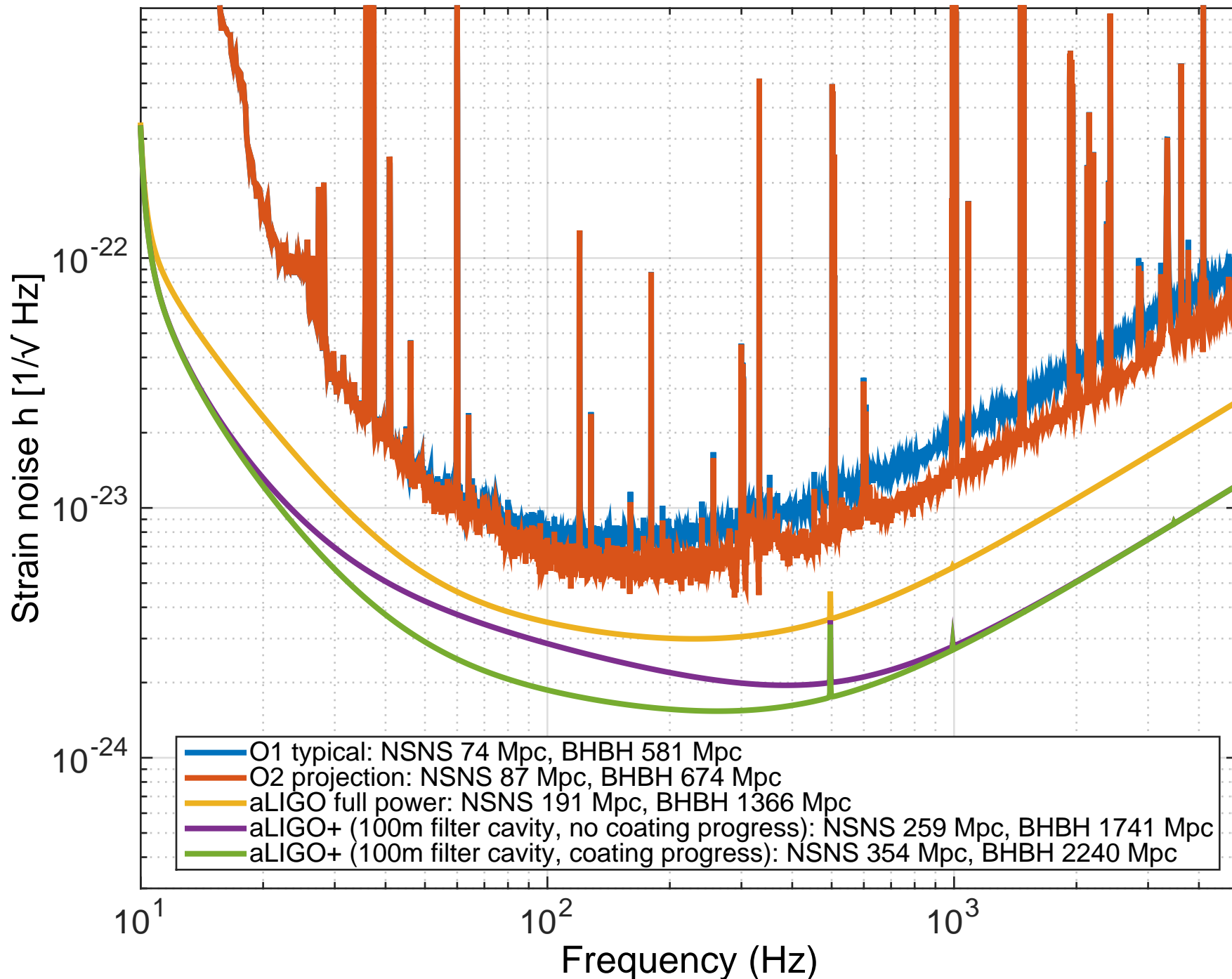
Projections toward aLIGO+ (Comoving Ranges: NSNS 1.4/1.4 M_{\odot} and BHBH 20/20 M_{\odot} )
