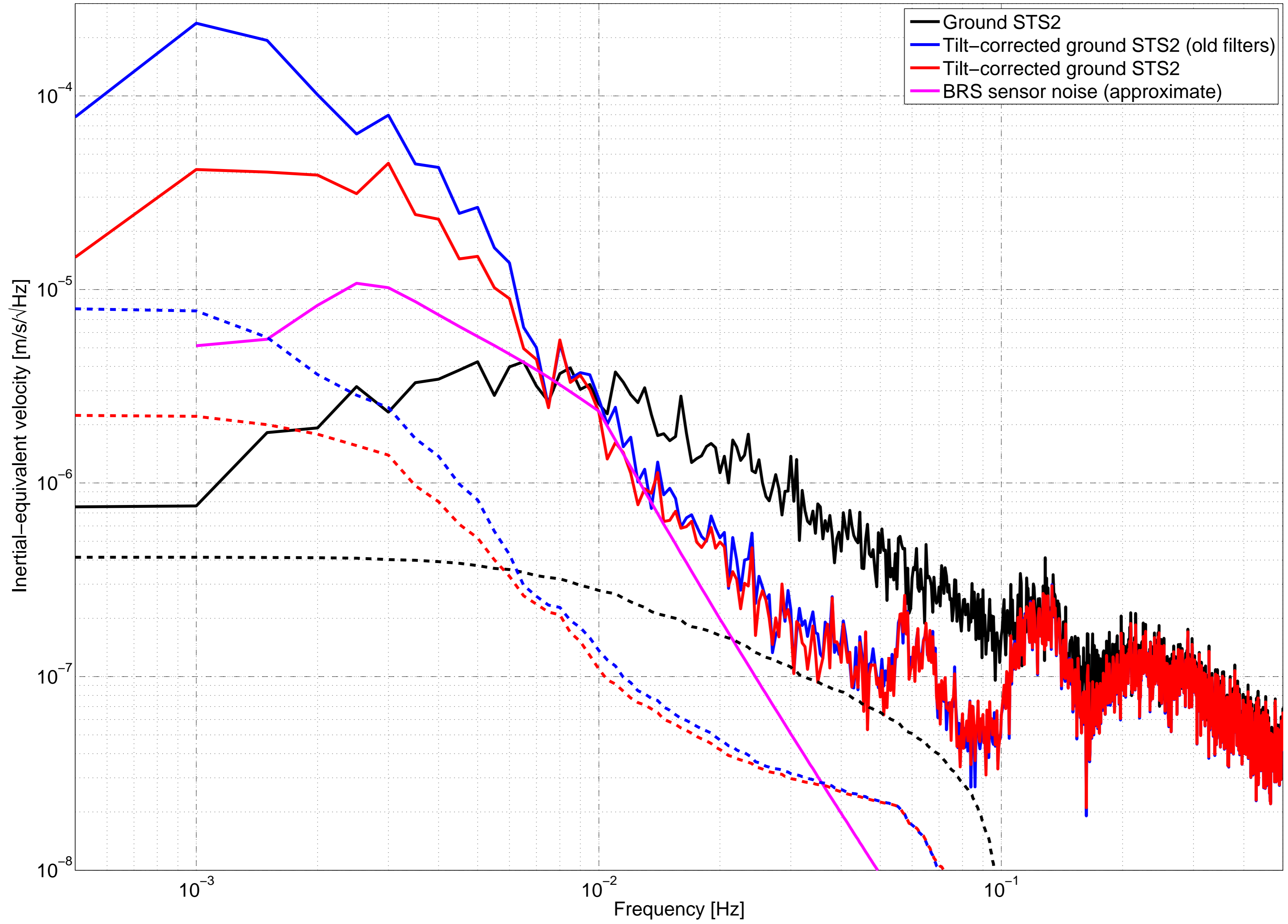
ETMY Tilt-correction filter tuning
