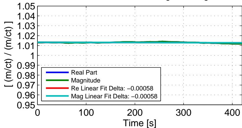
H1 TST Actuation Strength Change
