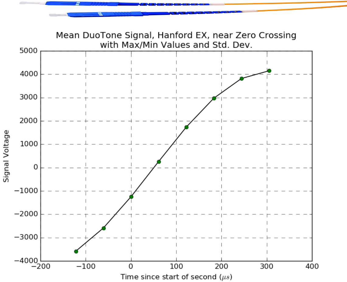
Figure 5: Zero crossing region of the second-to-second average of the DuoTone witness signals around the second edge at Hanford EX for the hour surrounding the G274296 event candidate. The line through the data points guide the eye to help visualize the zero crossing. Please note that the errors on each point are so small that they are covered by the circular symbol.
