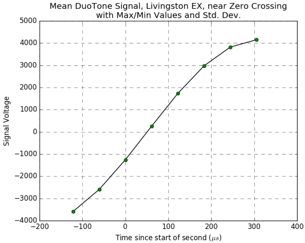
Figure 8: Zero crossing region of the second-to-second average of the DuoTone witness signals around the second edge at Livingston EX for the hour surrounding the G274296 event candidate. The line through the data points guide the eye to help visualize the zero crossing. Please note that the errors on each point are so small that they are covered by the circular symbol.
