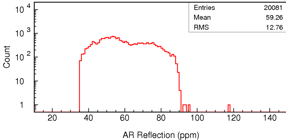
Fig. 1 ITM07 S2 AR reflection over a 160 mm diameter aperture.
