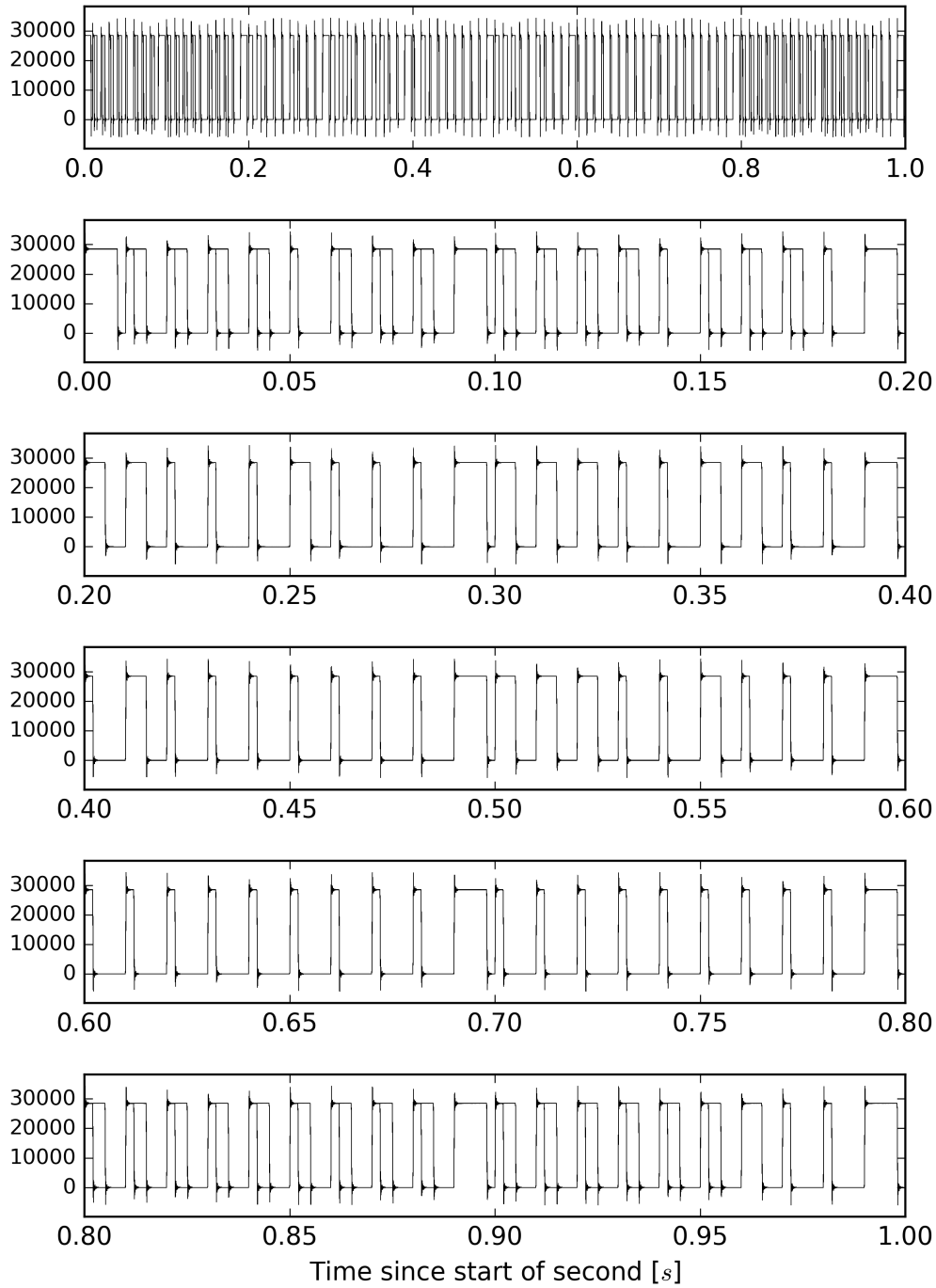
Overlay of L1:CAL-PCALX_IRIGB_OUT_DQ from 1187704734 to 1187704735
