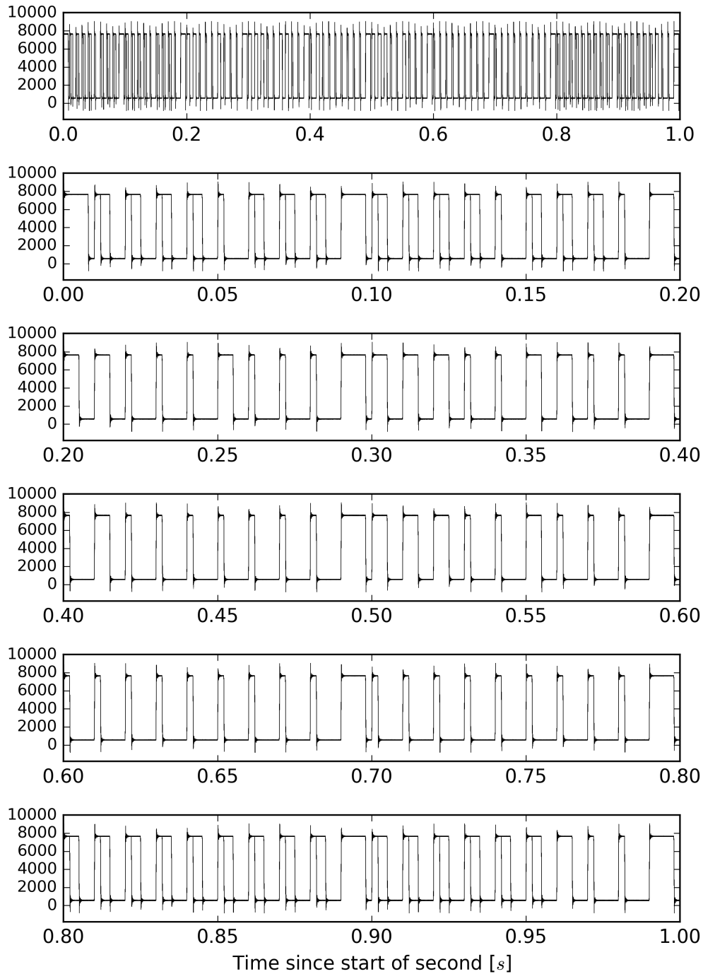
Overlay of H1:CAL-PCALX_IRIGB_OUT_DQ from 1187704734 to 1187704735
