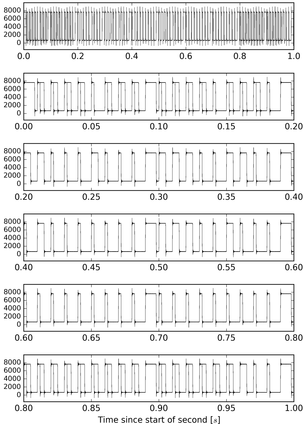
Overlay of H1:CAL-PCALY_IRIGB_OUT_DQ from 1187704734 to 1187704735
