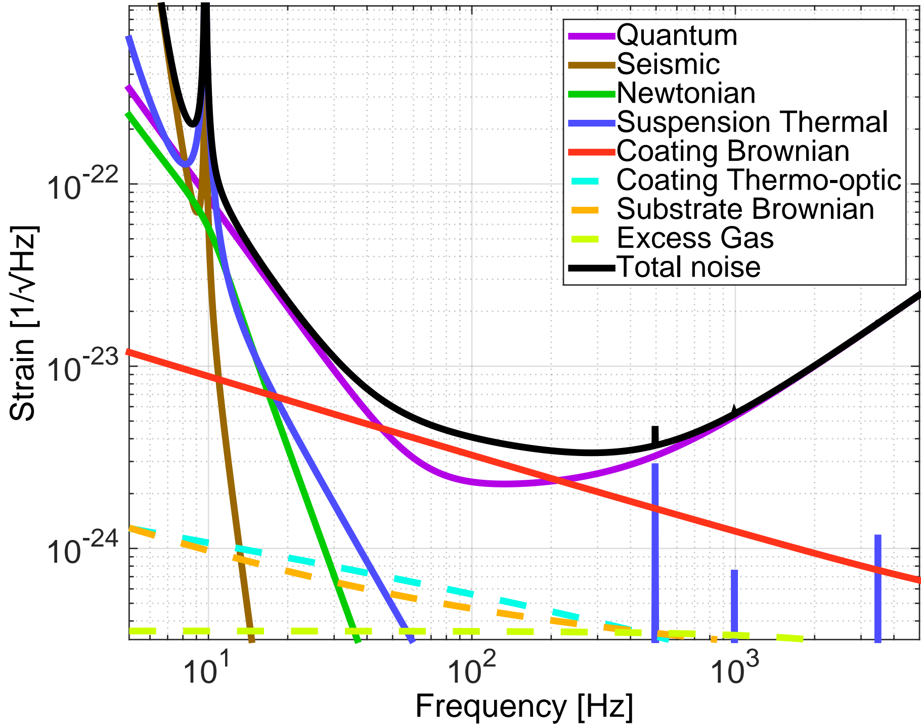
aLIGO new design curve: NSNS ( 1.4/1.4 M_{\odot} ) 173 Mpc and BHBH ( 30/30 M_{\odot} ) 1606 Mpc
