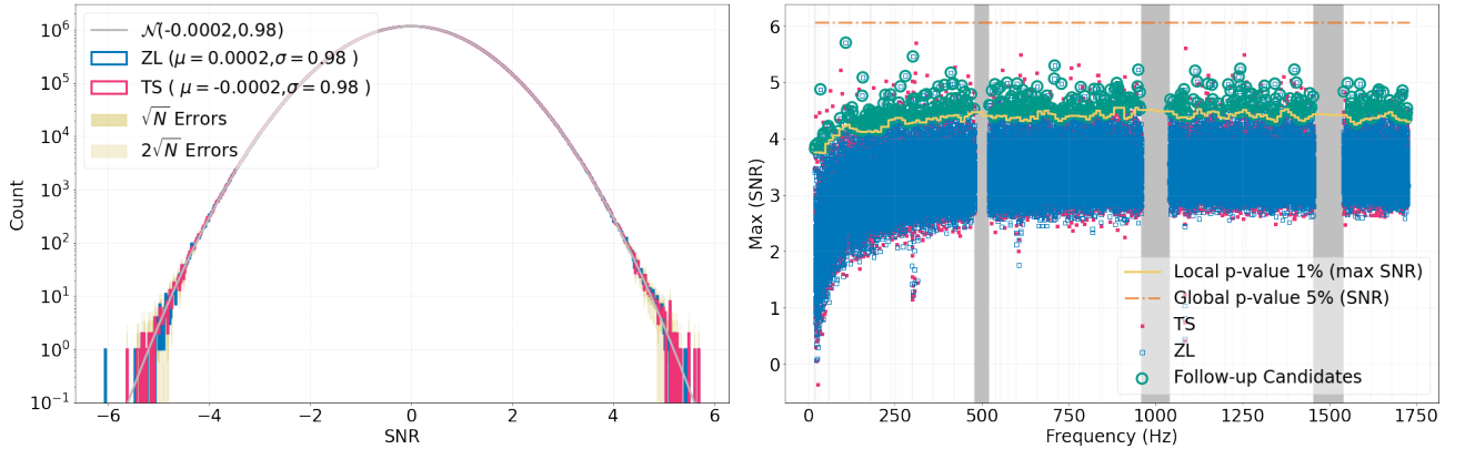
FIG. 2. Distributions of SNR from the O1+O2+O3 data set are shown in the left panel. The histogram of SNR from the time-shifted analysis is in red and from zero-lag analysis is in blue. Both the physical and unphysical time-shifted data set are consistent with Gaussian noise (grey histogram) within the 2\sigma error bars. The point with \text{SNR} \sim -6 is not astrophysically motivated and most likely caused by low number statistics (the two-tailed p -value is more than 5%). Right panel depicts the distribution of maximum SNRs from both time-shifted (TS) and zero-lag (ZL) analyses performed over the O1+O2+O3 data set as a function of frequency. The grey solid lines represent the frequencies that are notched in the data set. The yellow curve shows the 99th percentile of maximum SNR for every 10 Hz frequency bin in the time-shifted analysis, smoothed over 3 neighboring 10 Hz bins. The orange dot-dashed line delineates the trials-factor-corrected, one-sided global p -value of 5%. Though we do not find any outliers significantly above the noise background, the teal circles represent 515 candidates which may be followed up by a more sensitive matched-filtering-based analysis.
